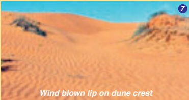
Wind blown lip on dune crest
